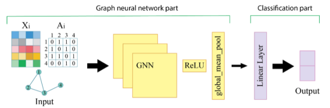
Figure 4. General Architecture of a GNN-Based Classification Model
